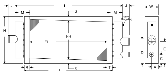
Figure 6 - RA, TA Dimension Info
