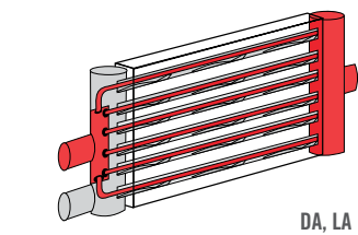
Figure 3 - DA, LA Steam Distribution
