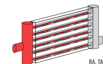
Figure 5 - RA, TA Steam Distribution
