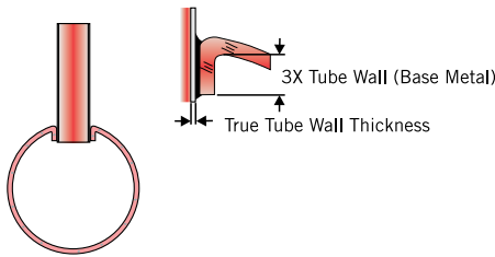
Figure 12 - Cu Tubes to Cu Header Joint
