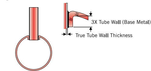
Figure 12 - Cu Tubes to Cu Header Joint
