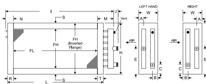
Figure 10 - SS, SH Dimension Info
