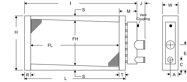
Figure 2 - JA, GA Dimension Info
