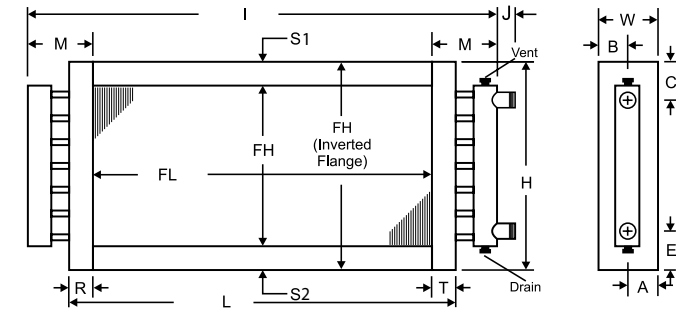
Figure 5 - Opposite End Connections
