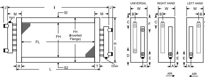
Figure 4 - Collection Header - Same End Connections
