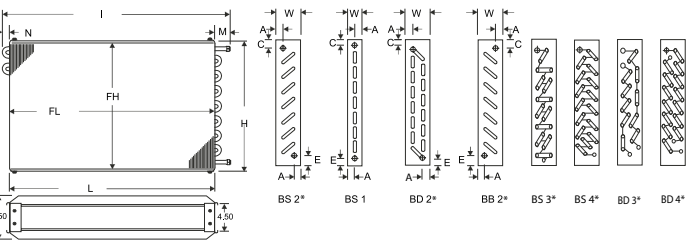
Figure 6 - Booster Coil - Slip & Drive shown
