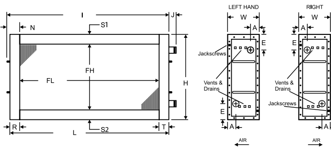
Figure 11 - Cleanable Both Ends - Opposite End Connections
