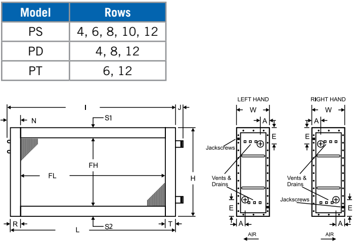
Figure 16 - Cleanable Supply End - Same End Connections
