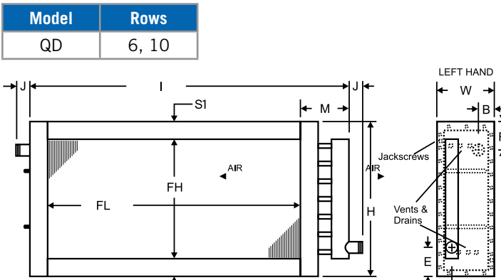
Figure 14 - Cleanable Opposite Supply End - Opposite End Connections
