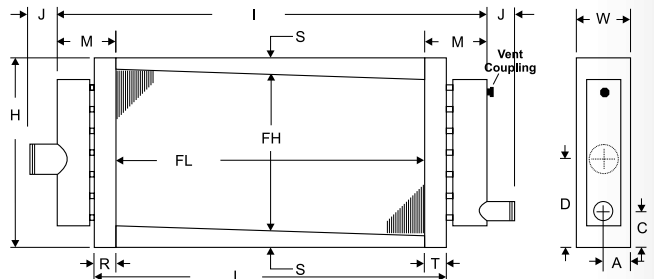
Figure 8 - SA, HA, SB, HB Dimension Info
