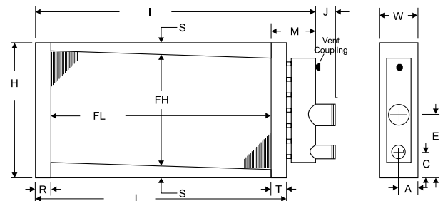
Figure 2 - JA, GA Dimension Info
