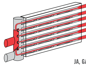
Figure 1 - JA, GA Steam Distribution
