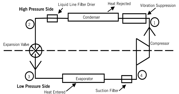
Figure 2 - General Plumbing
