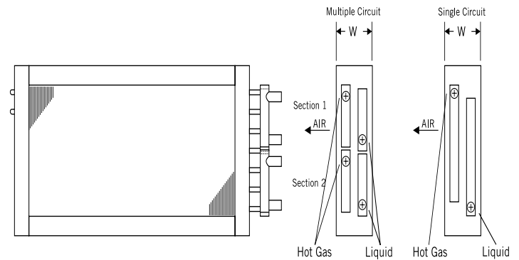
Figure 1 - Condenser Coils
